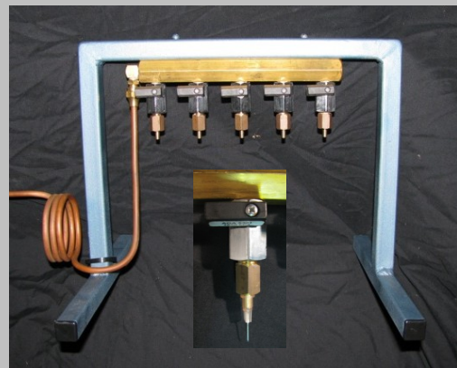
VACUUM MANIFOLD Extraction of multiple vials for sample collection when connected to vacuum pump
